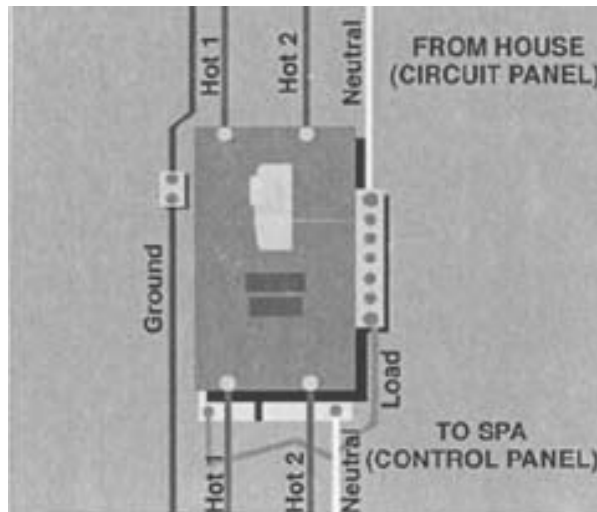
Figure 2. GFCI Hook-Up.
